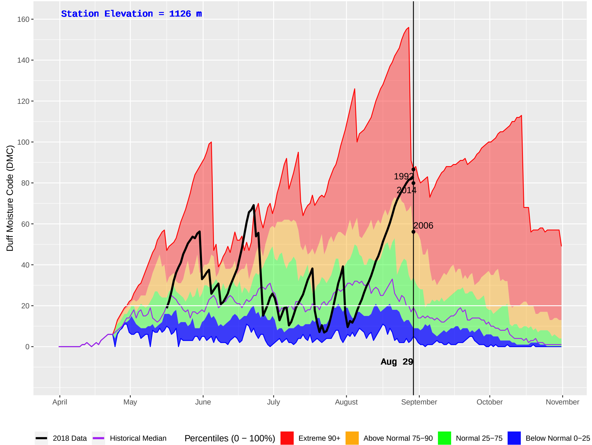
BLACKPINE (148) : Historical (1980–2016) and Current (2018) Daily Duff Moisture Code (DMC)
