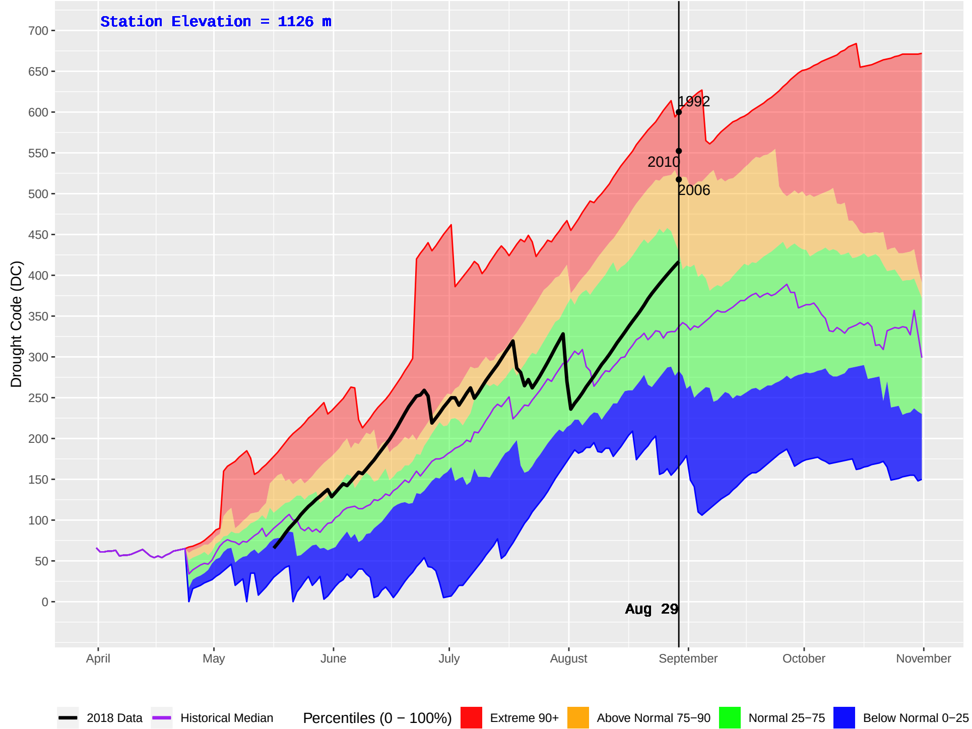
BLACKPINE (148) : Historical (1980–2016) and Current (2018) Daily Drought Code (DC)
