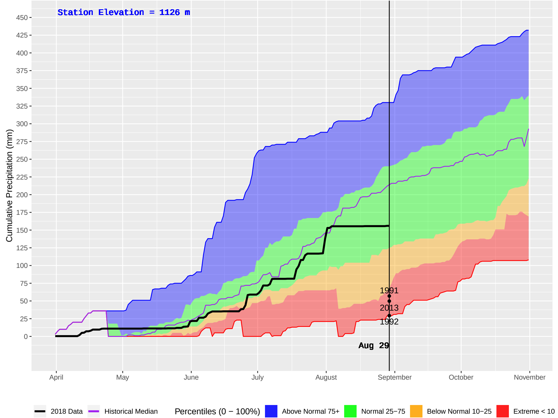
BLACKPINE (148) : Historical (1980–2016) and Current (2018) Daily Cumulative Precipitation
