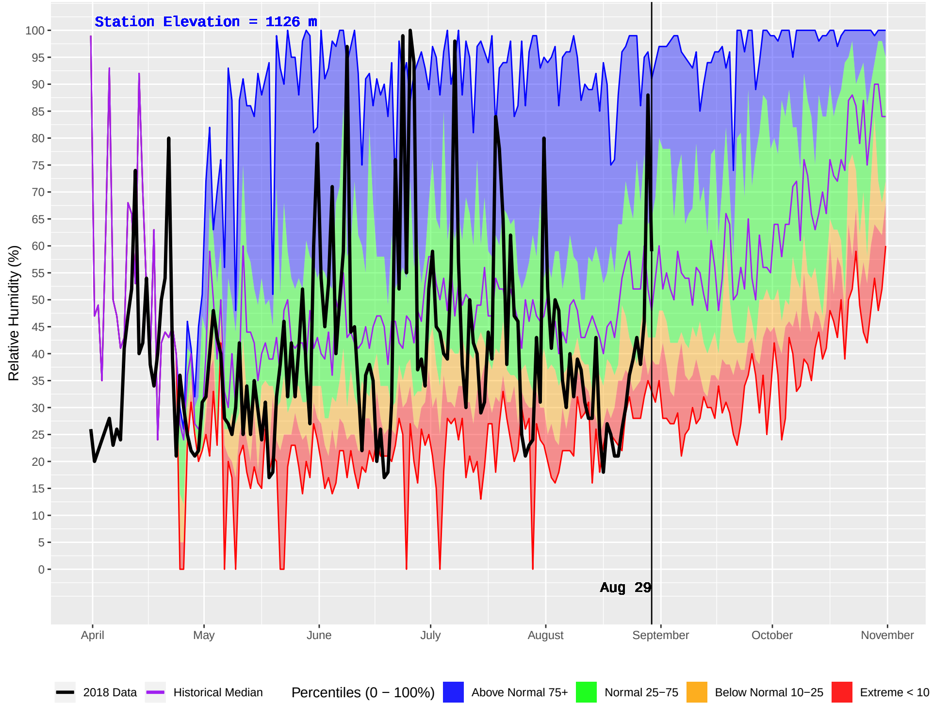
BLACKPINE (148) : Historical (1980–2016) and Current (2018) Daily Relative Humidity
