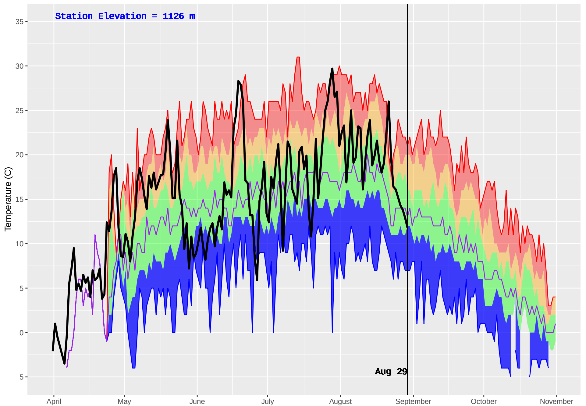
BLACKPINE (148) : Historical (1980–2016) and Current (2018) Daily Temperature
