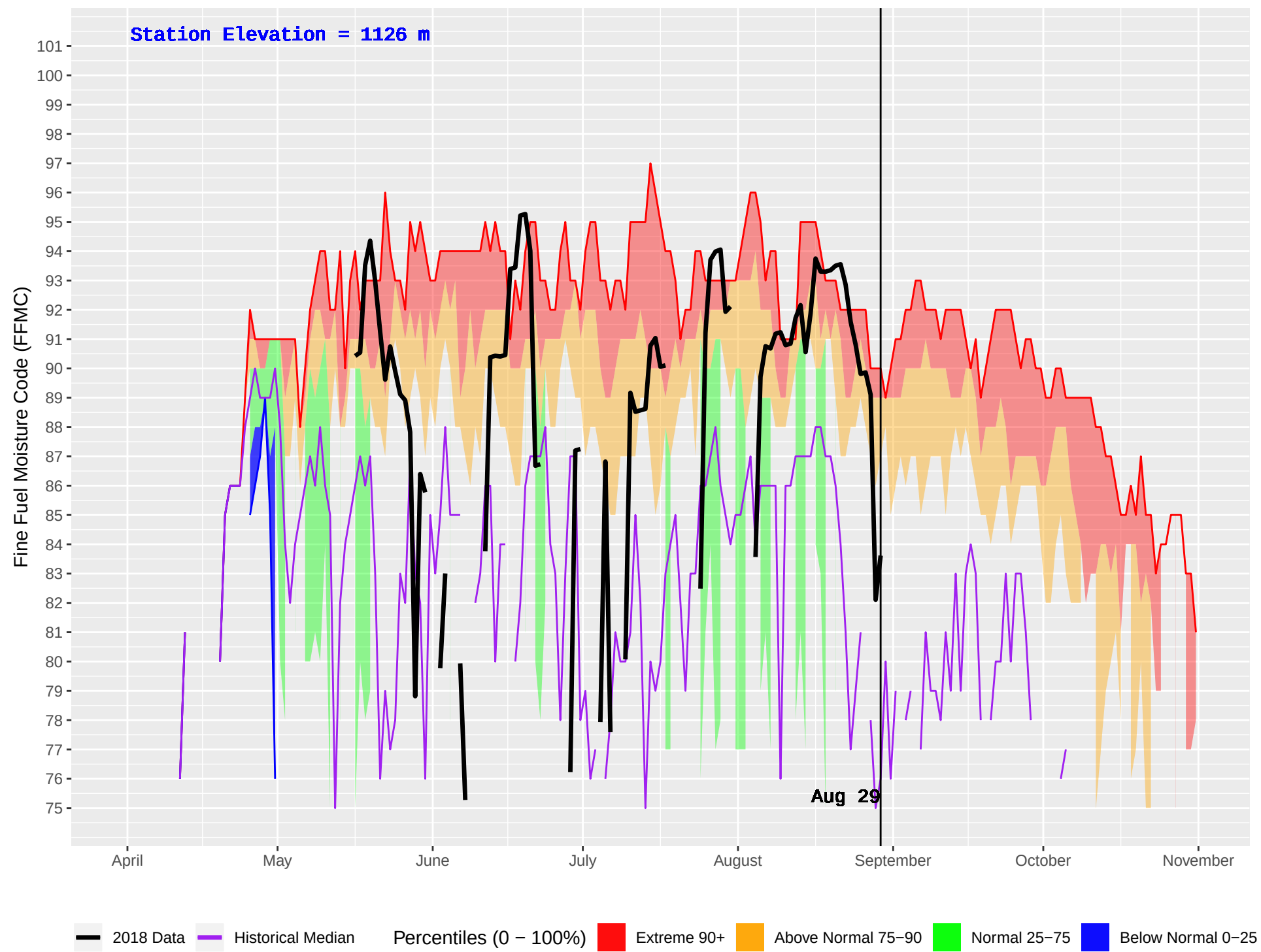
BLACKPINE (148) : Historical (1980–2016) and Current (2018) Daily Fine Fuel Moisture Code (FFMC)
